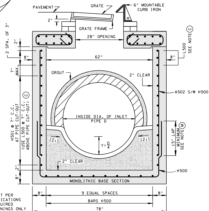
SECTION B-B
