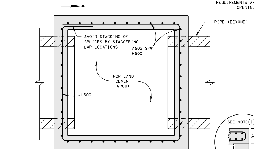
SECTION E-E
